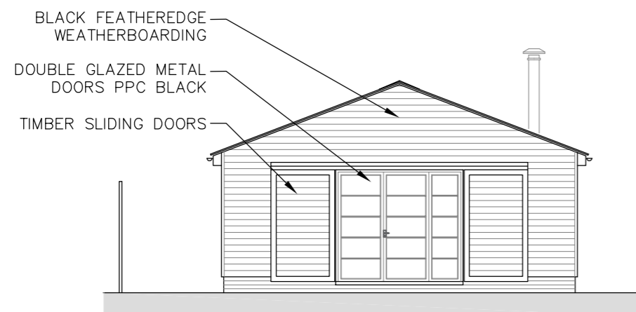
EAST (REAR) ELEVATION
