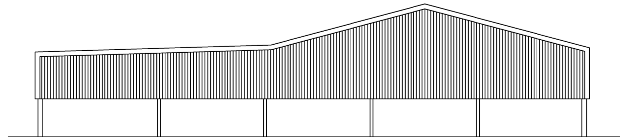
North Elevation
