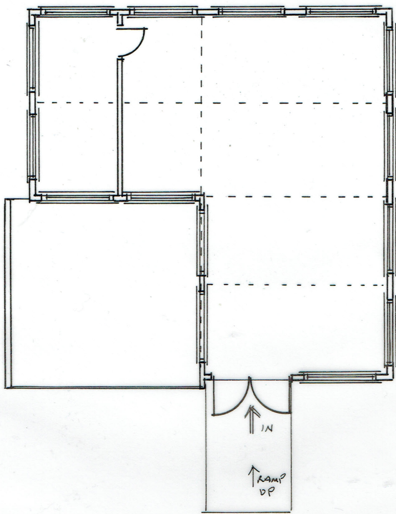
EXISTING GROUND FLOOR PLAN OF FORMER AGRICULTURAL BUILDING.
